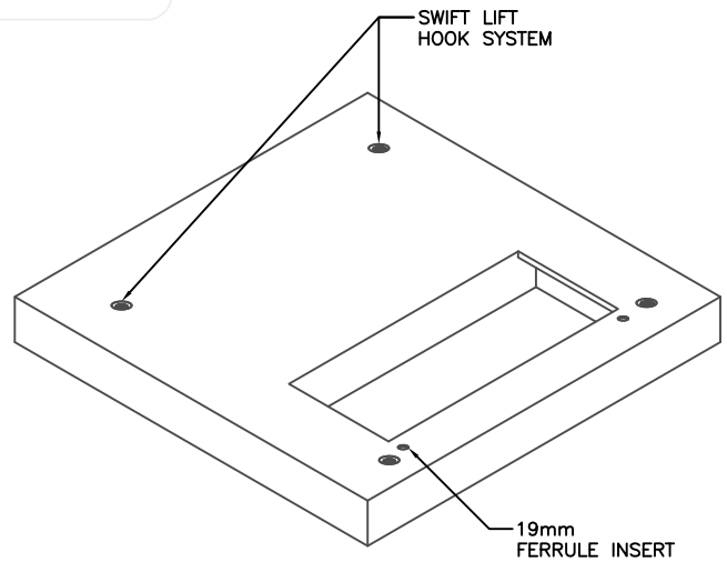
ISOMETRIC VIEW
