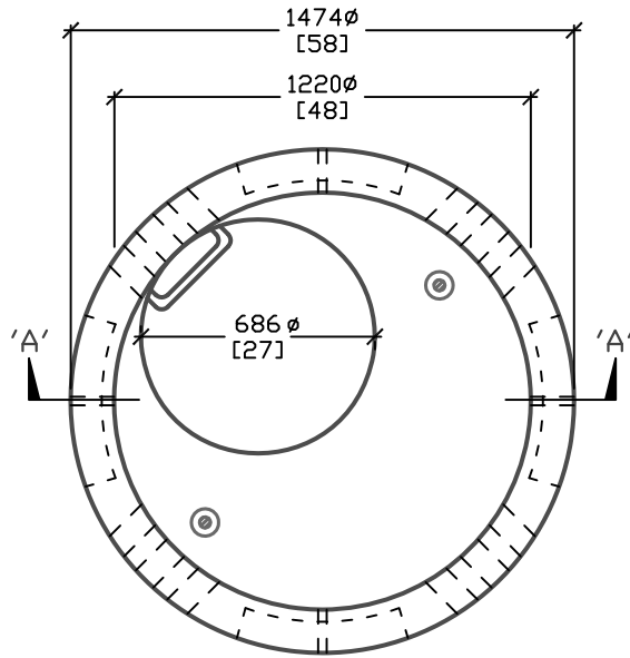
PLAN VIEW
