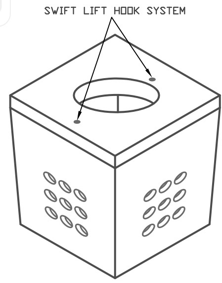
ISOMETRIC VIEW
