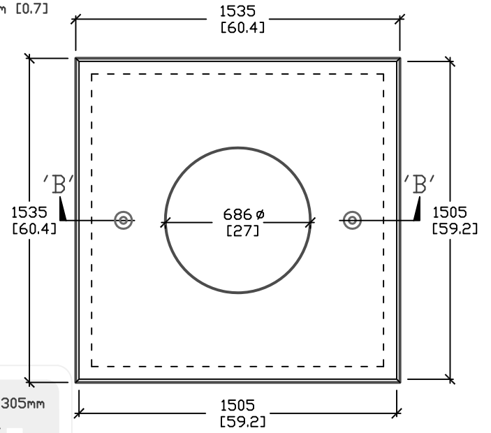
PLAN VIEW (PAD)
