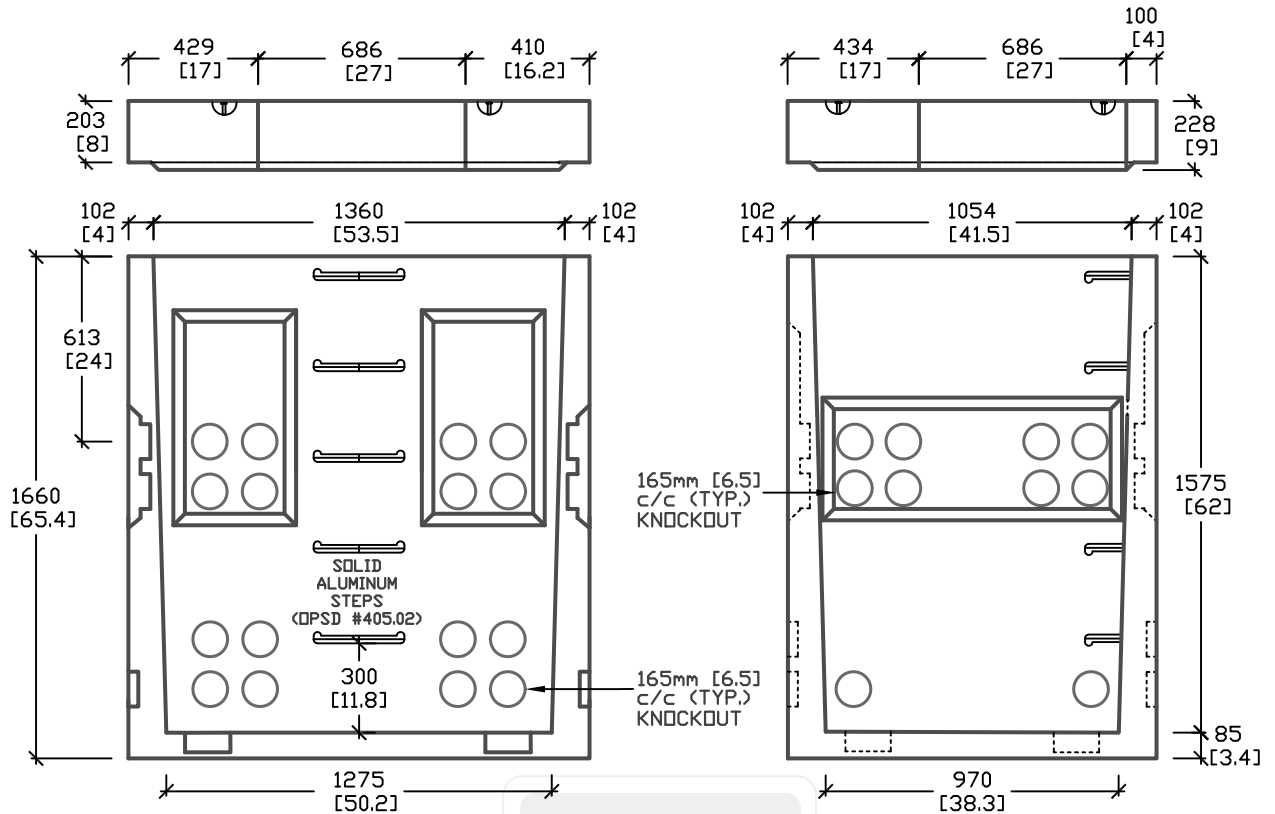
CROSS SECTION 'A'
