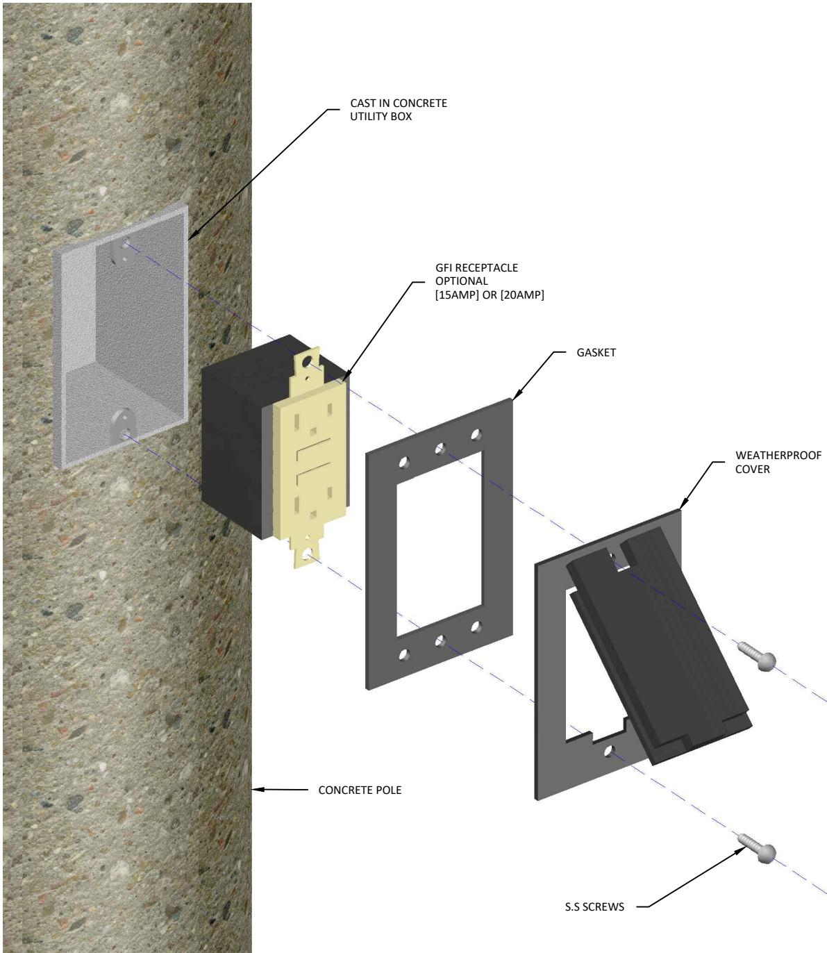
GFI MOUNTING DETAIL
