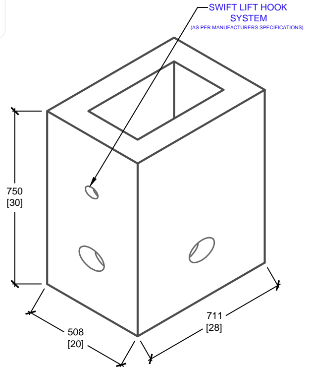
ISOMETRIC VIEW
