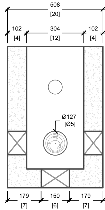
CROSS SECTION 'B'
