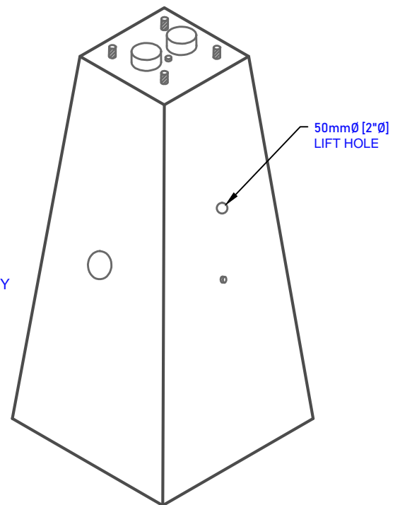
ISOMETRIC VIEW
