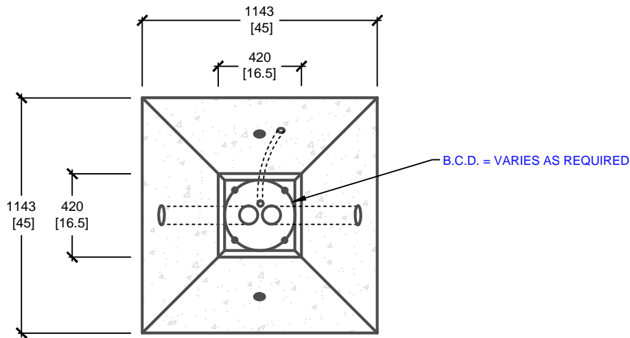
PLAN VIEW
