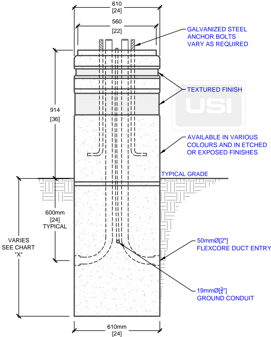
SIDE ELEVATION
